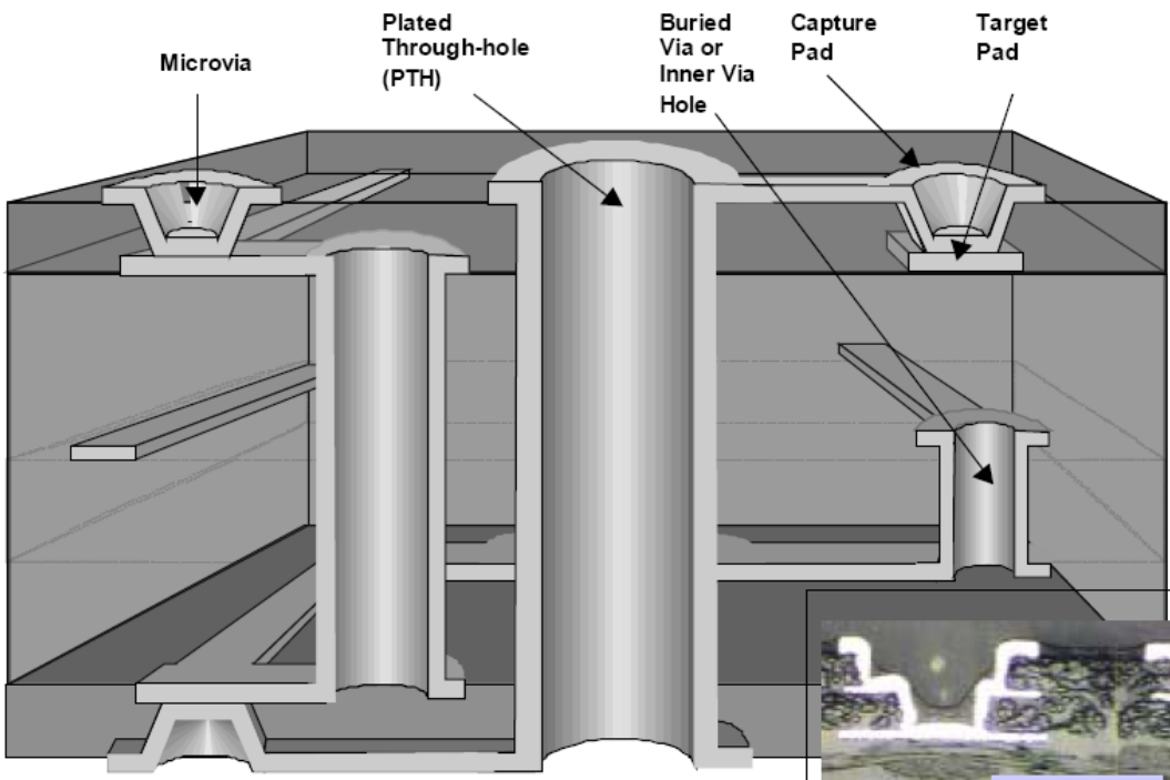
1A: Schematic
